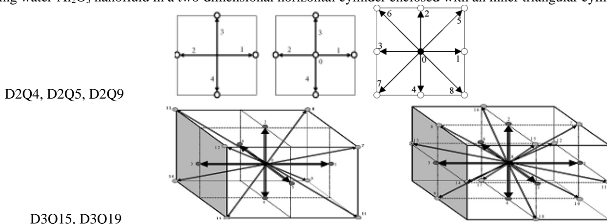
Figure 1. Lattice arrangements
